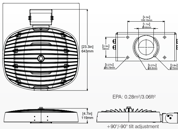
YOKE MOUNT (SPX-BKT-AR-YM): 16.8 kg | 37 lbs
