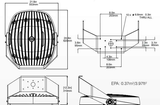
HIGH VIBRATION YOKE (SPX-BKT-AR-YK): 23.8 kg | 52.5 lbs
