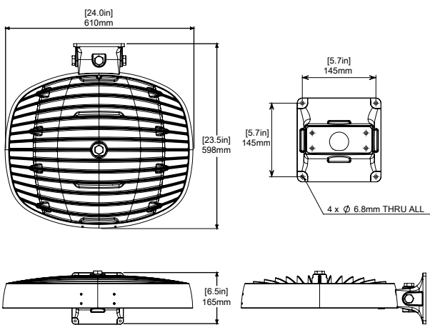
YOKE MOUNT (SPX-BKT-AR-YM): 16.8 kg | 37 lbs
