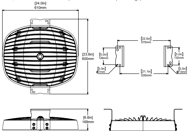
SURFACE/SUSPENDED MOUNT (SPX-BKT-AR-SM-GY): 16.8 kg | 37 lbs
