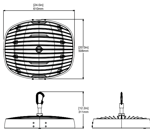
HANGING PENDANT (SPX-BKT-AR-HK): 16.4 kg | 36 lbs
