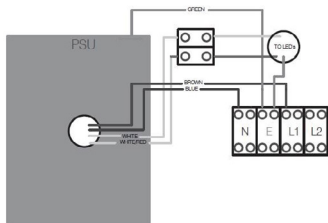
Typical wiring diagram - Standard Variants
