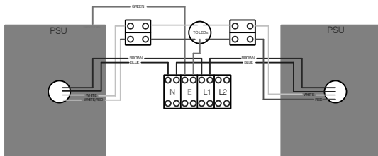
Typical wiring diagram - Standard Variants
